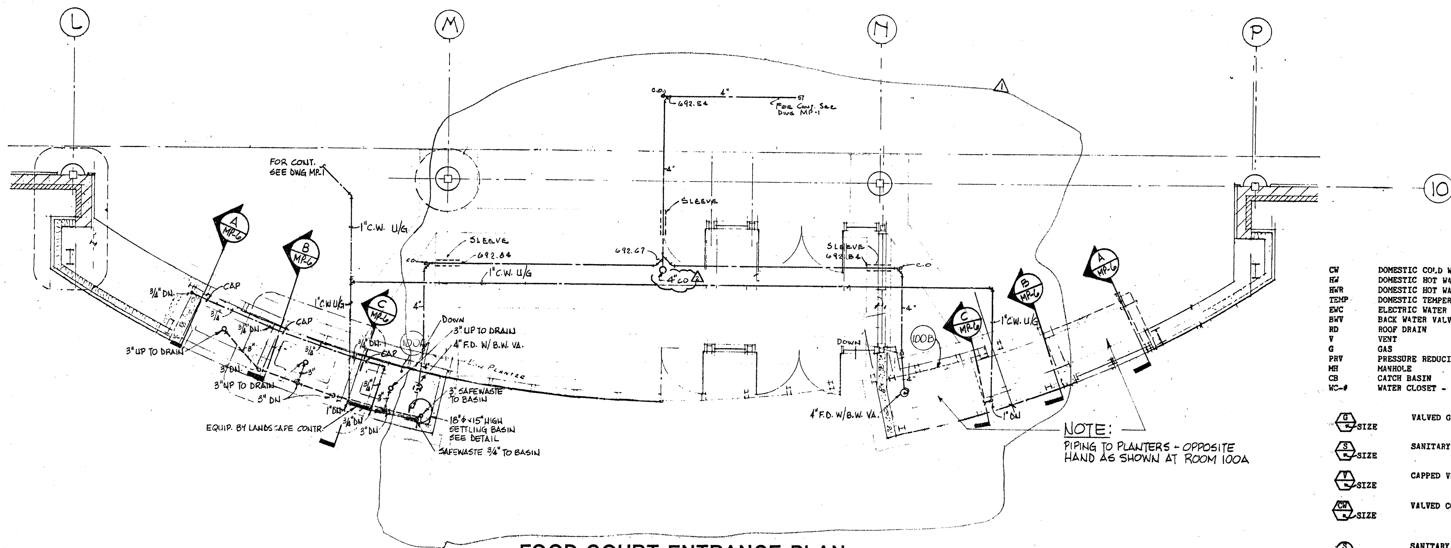
FOOD COURT ENTRANCE PLAN
