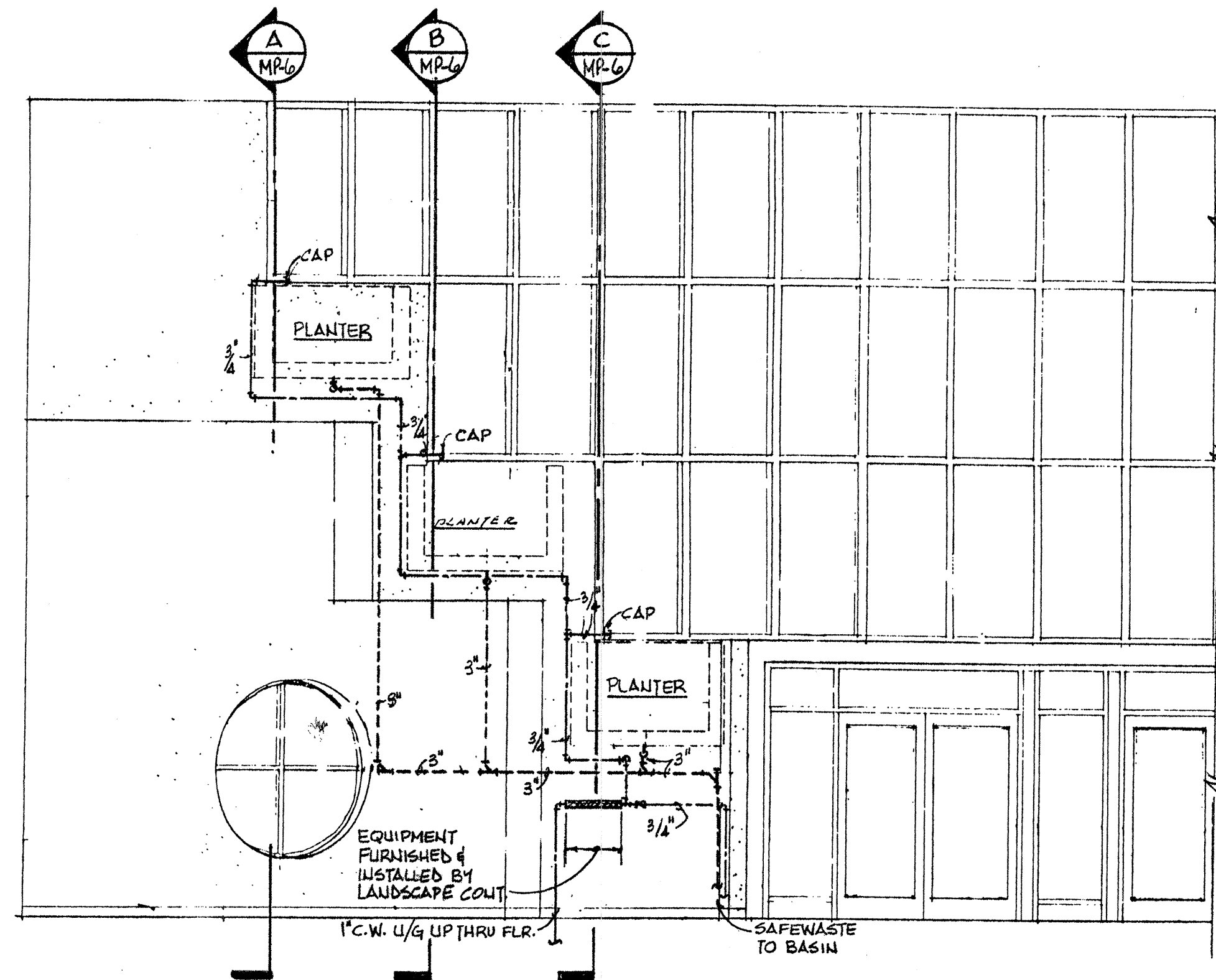
HALF ELEVATION - INTERIOR
